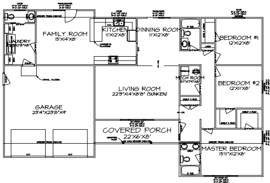
FIRST FLOOR PLAN SCALE: 1/4"=1'-0" FLOOR PLAN NOTES: 1. ALL INTERIORS SHALL BE 5/8\"/>
