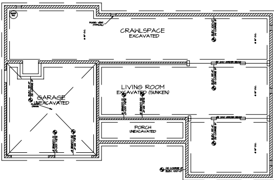
FOUNDATION PLAN SCALE: 1/4"=1'-0" FOUNDATION PLAN NOTES: 1. FOUNDATION SHALL BE CONCRETE ON GRAVEL FILL. 2. ALL FOUNDATION SHALL BE 12" MIN. THICK. 3. ALL FOUNDATION SHALL BE 4" MIN. COVER. 4. ALL FOUNDATION SHALL BE 4" MIN. COVER. 5. ALL FOUNDATION SHALL BE 4" MIN. COVER. 6. ALL FOUNDATION SHALL BE 4" MIN. COVER. 7. ALL FOUNDATION SHALL BE 4" MIN. COVER. 8. ALL FOUNDATION SHALL BE 4" MIN. COVER. 9. ALL FOUNDATION SHALL BE 4" MIN. COVER. 10. ALL FOUNDATION SHALL BE 4" MIN. COVER.
